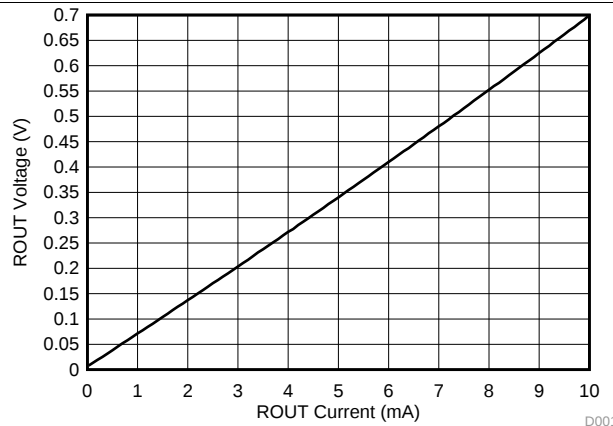
Figure 1. Receiver VOL vs Output Current
