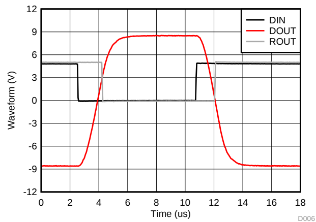
120 kbit/s, 1-nF load Figure 13. Driver and Receiver Loopback Signal
