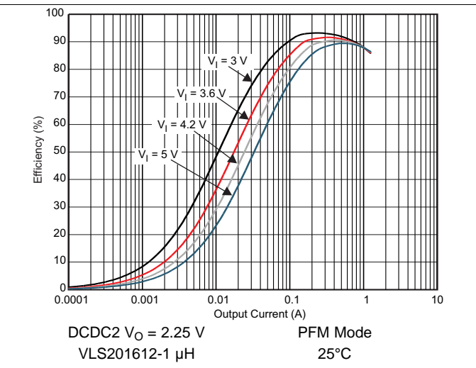
Figure 5-10. DCDC2 Efficiency vs Output Current / PFM Mode
