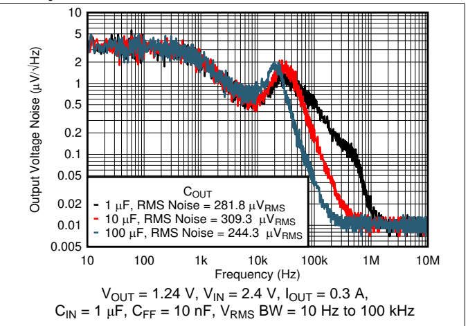
图 26. Output Noise ( V_n ) vs Frequency and C_{OUT}
