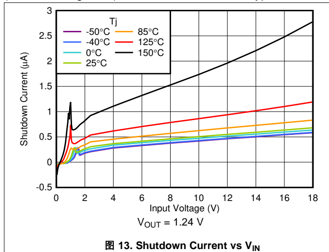
图 13. Shutdown Current vs V_{IN}
