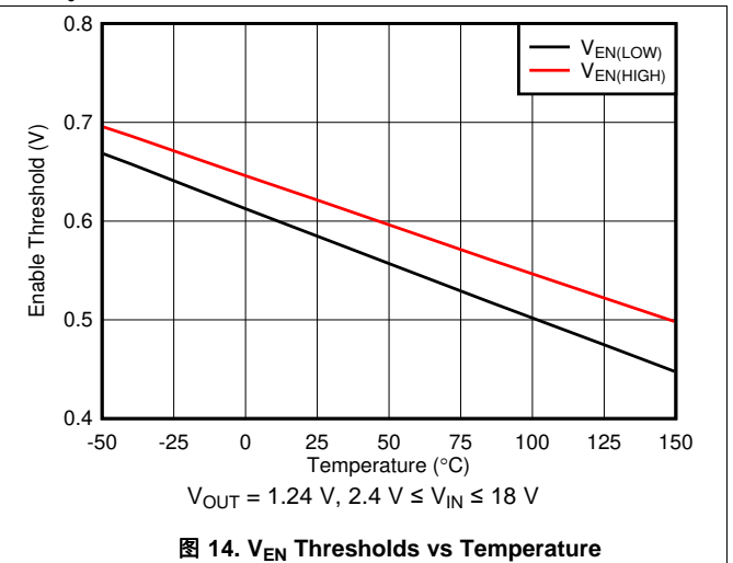
图 14. V_{EN} Thresholds vs Temperature
