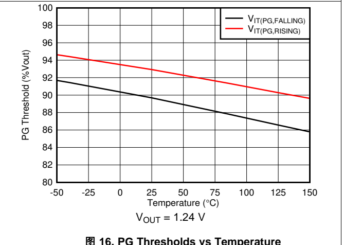
图 16. PG Thresholds vs Temperature
