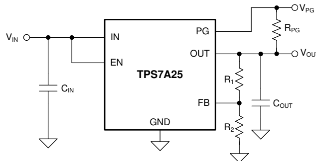
图 40. Generating a 5-V Rail From a Multicell Power Bank
