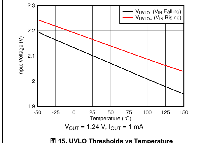
图 15. UVLO Thresholds vs Temperature
