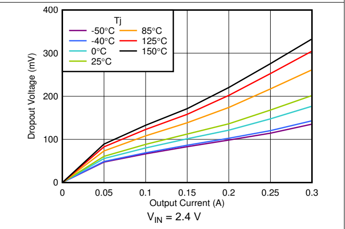
图 6. Dropout Voltage vs I_{IN}
