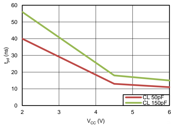
Figure 1. Propagation Delay
