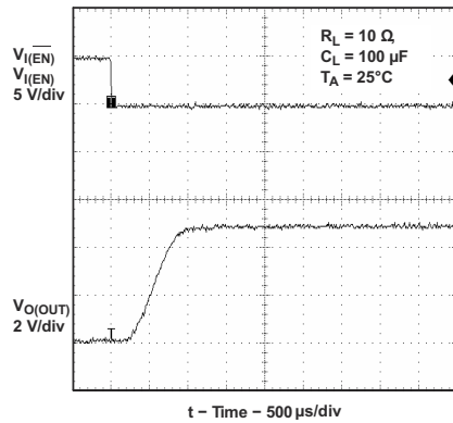
Figure 9-5. Turnon Delay and Rise Time With 100-μF Load
