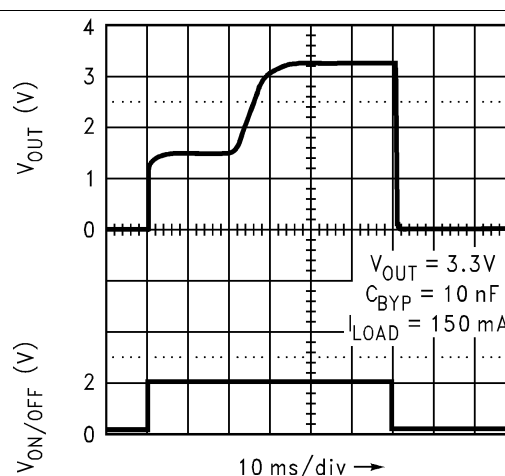
Figure 38. Turnon Time
