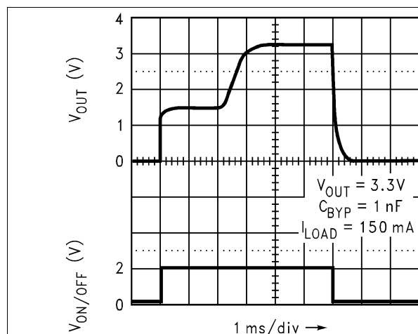
Figure 37. Turnon Time
