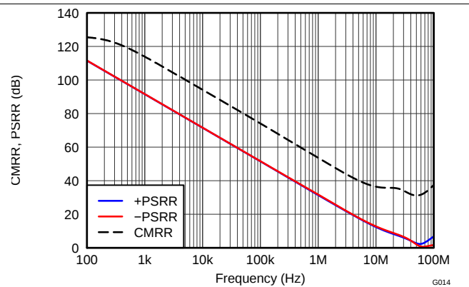
图 14. CMRR and PSRR vs Frequency (Referred to Input)
