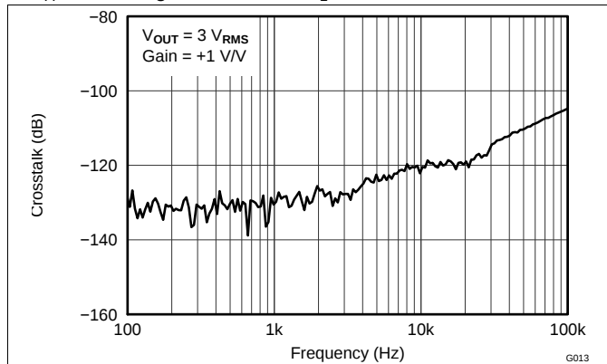
图 13. Channel Separation vs Frequency
