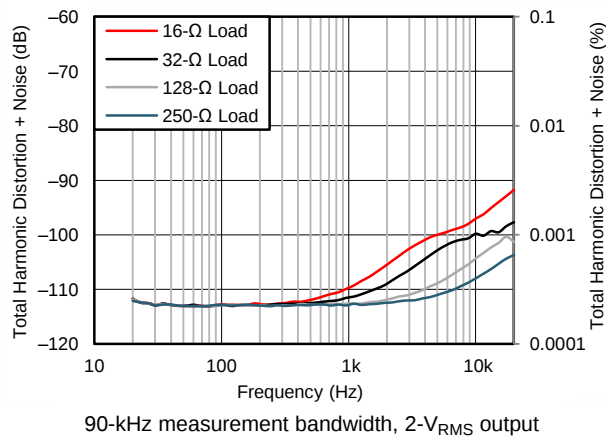
图 44. THD+N vs Frequency for Various Loads
