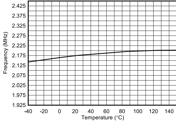
12 V IN 2.2 MHz 图 6-55. Oscillator Frequency vs Temperature
