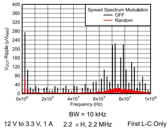
图 6-12. V_{OUT} Ripple FFT After the First L-C Filter
