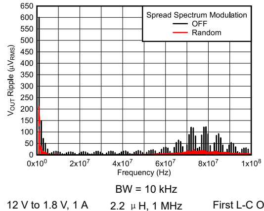
图 6-8. V_{OUT} Ripple FFT After the First L-C Filter
