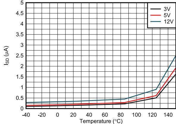
V IN : 3 V, 5 V, 12 V 图 6-56. Shutdown Current vs Temperature
