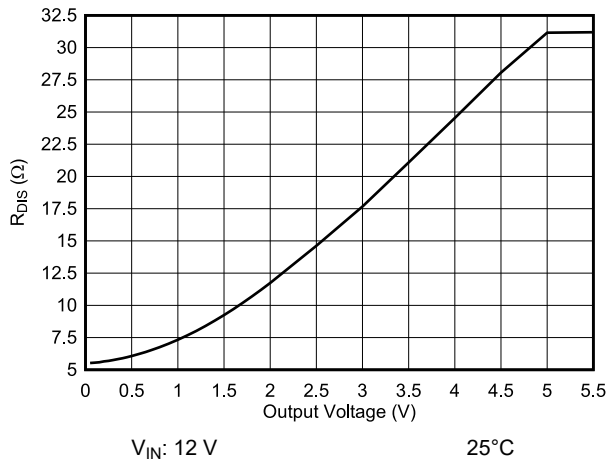
V IN : 12 V 25°C 图 6-57. Output Discharge Resistance vs Output Voltage
