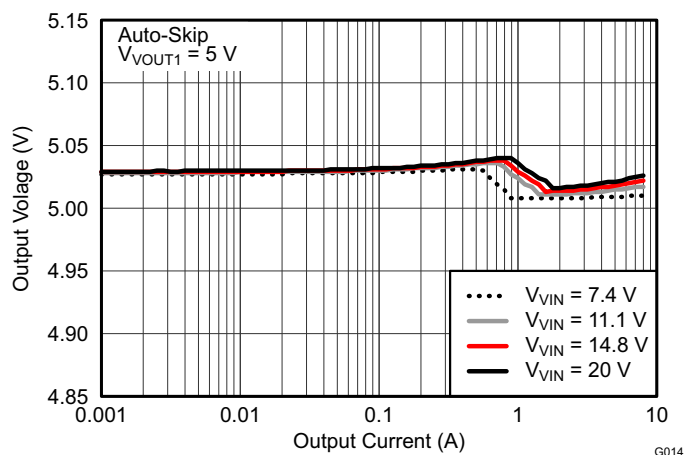
Figure 13. Load Regulation
