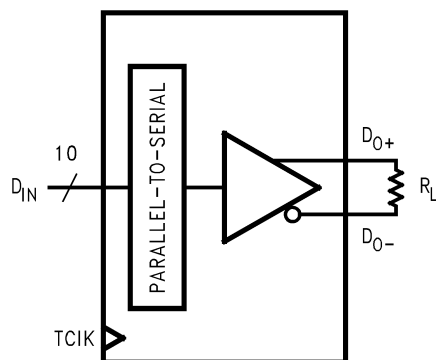
Figure 18. V_{OD} Diagram
