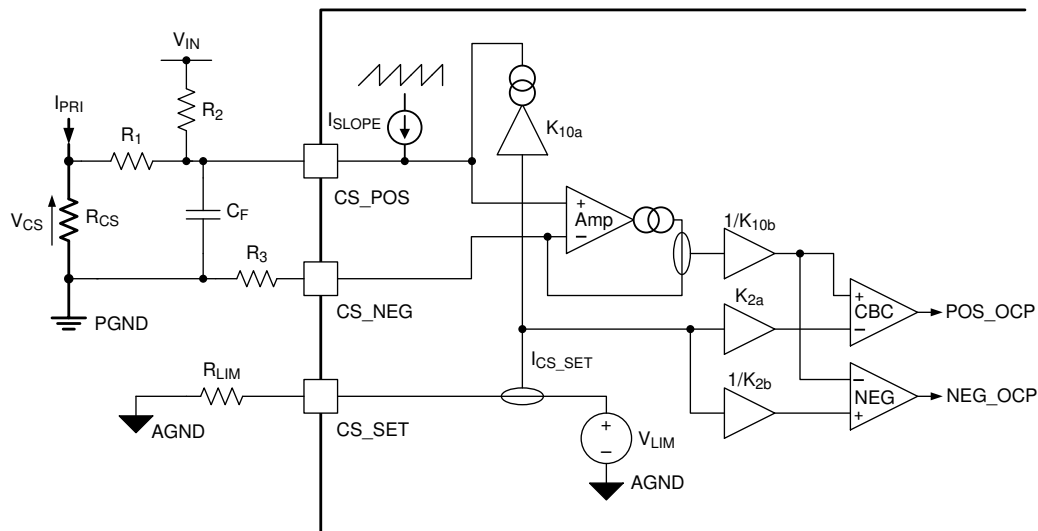
图 7-12. Block Diagram of the Current Limiting Function
