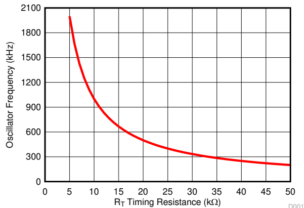
图 6-5. Oscillator Frequency vs R_T Timing Resistance
