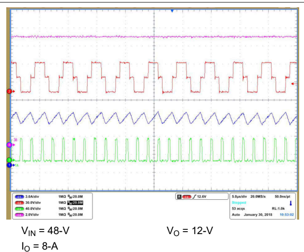
图 8-14. Steady State Operation Waveform
