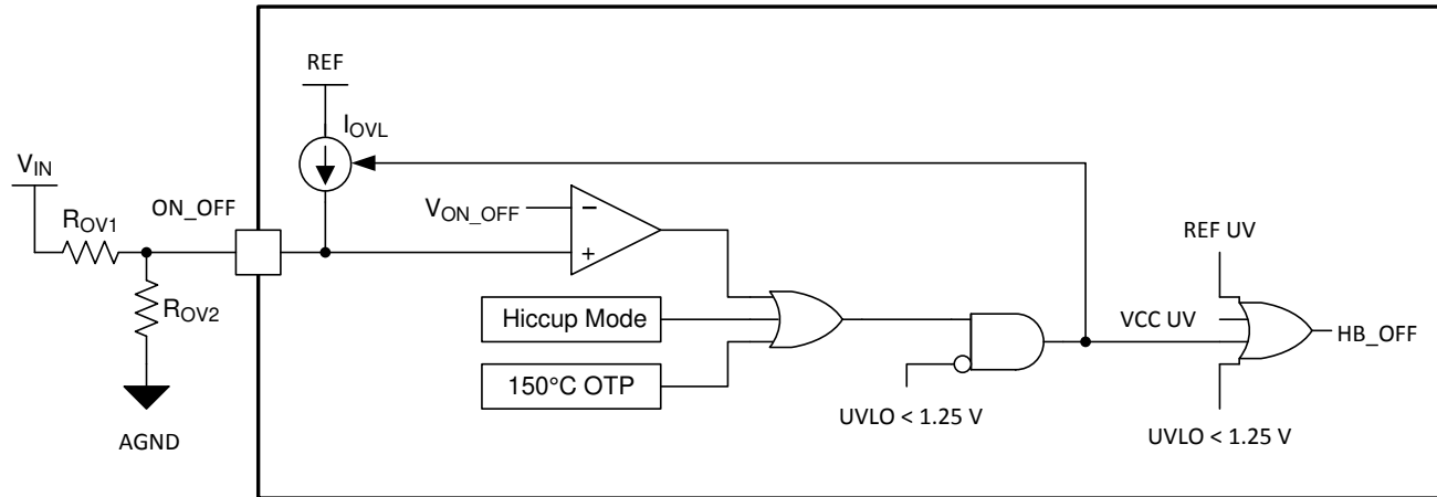
图 7-21. ON/OFF Pin Configured as OVP Pin
