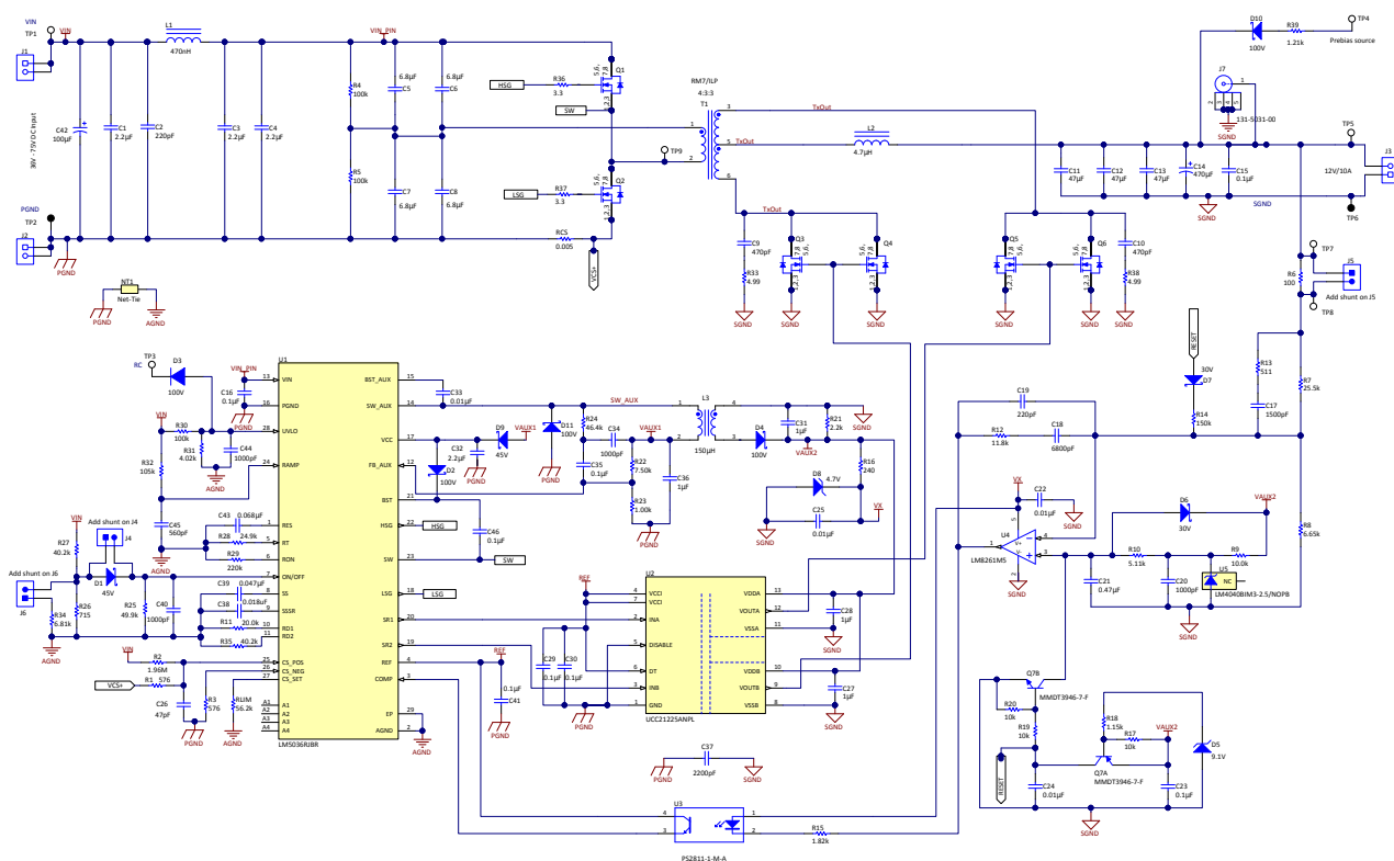
图 8-1. Evaluation Board Schematic
