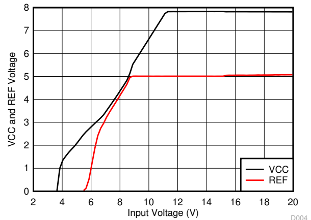
图 6-4. VCC and REF Voltage vs Input Voltage
