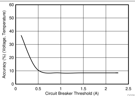
Figure 23. Circuit Breaker Threshold Accuracy vs Circuit Breaker Threshold I_{\text{CB}}
