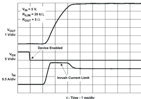
图 25. Turn on Delay and Rise Time
