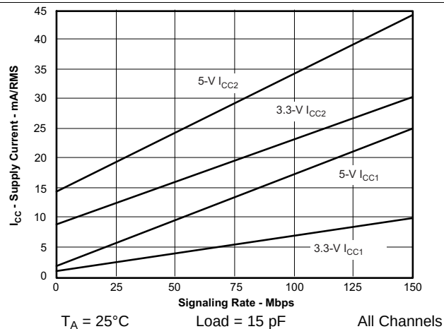
Figure 3. ISO7240C/M RMS Supply Current vs Signaling Rate
