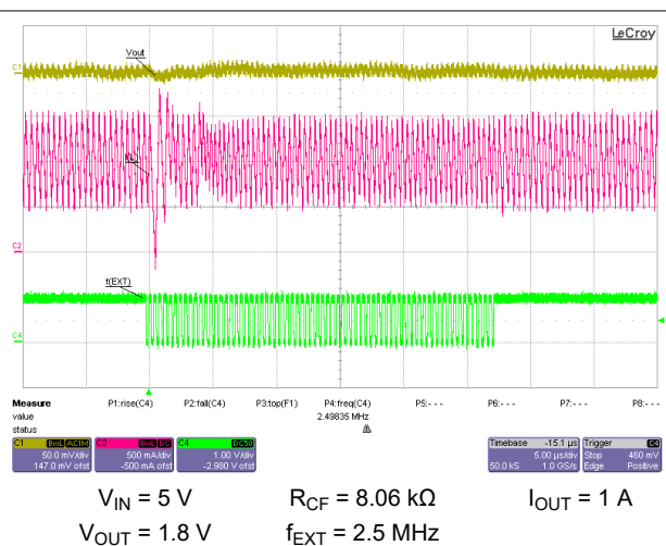
图 10-62. Switching from External Synchronization to Internal Fixed Frequency
