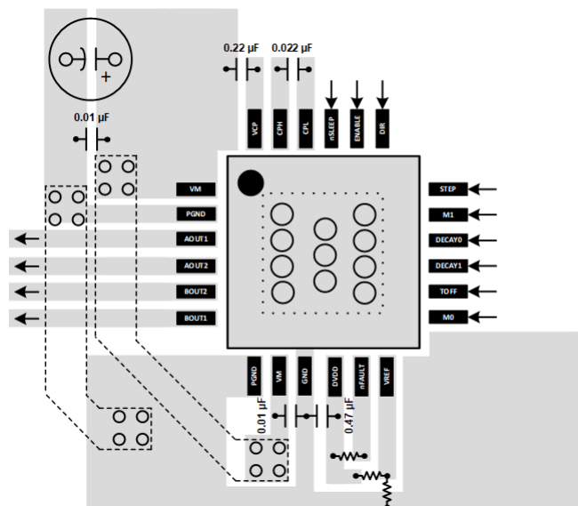
Figure 10-2. QFN Layout Example
