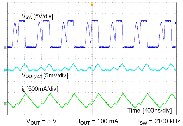
Figure 24. DCM Mode
