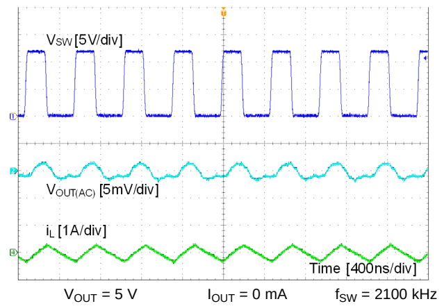
Figure 26. FPWM Mode
