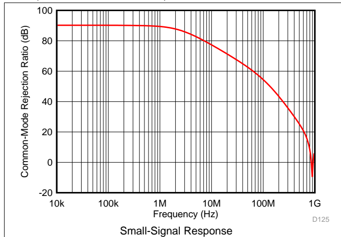
图 25. Common-Mode Rejection Ratio vs Frequency
