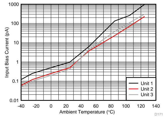
图 38. Input Bias Current vs Ambient Temperature
