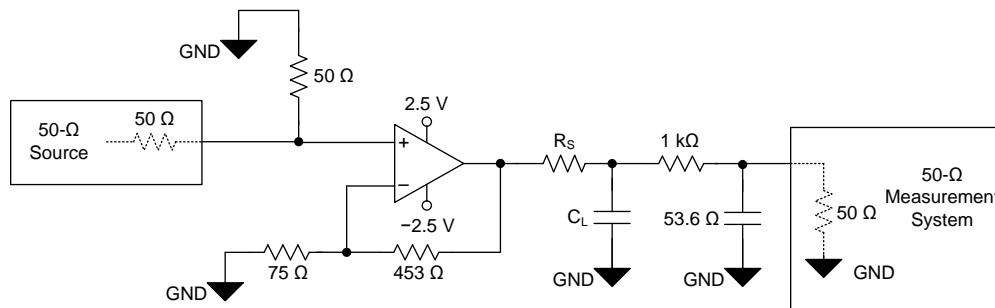
图 45. Capacitive Load Driver Configuration
