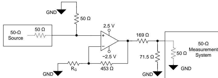
图 43. Noninverting Configuration
