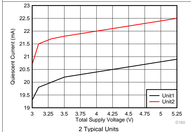
图 27. Quiescent Current vs Supply Voltage
