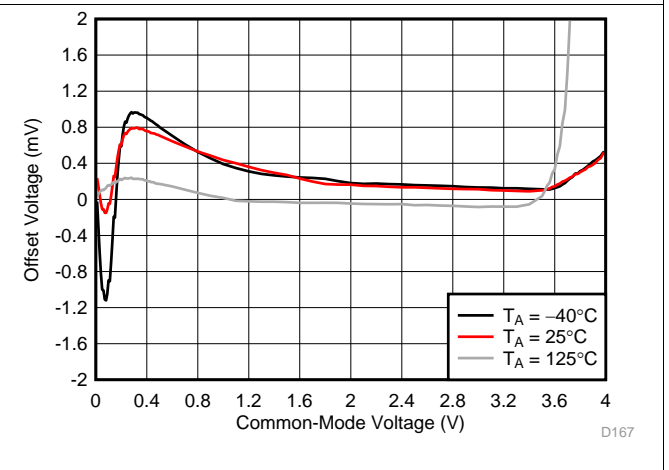
图 34. Offset Voltage vs Input Common-Mode Voltage vs Ambient Temperature
