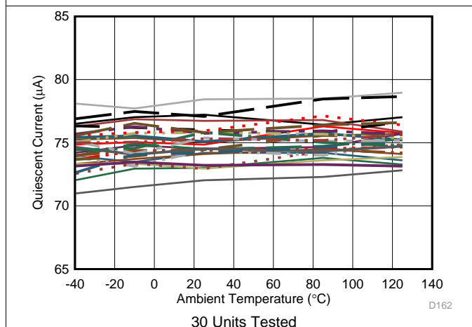
图 29. Quiescent Current (Amplifier Disabled) vs Ambient Temperature
