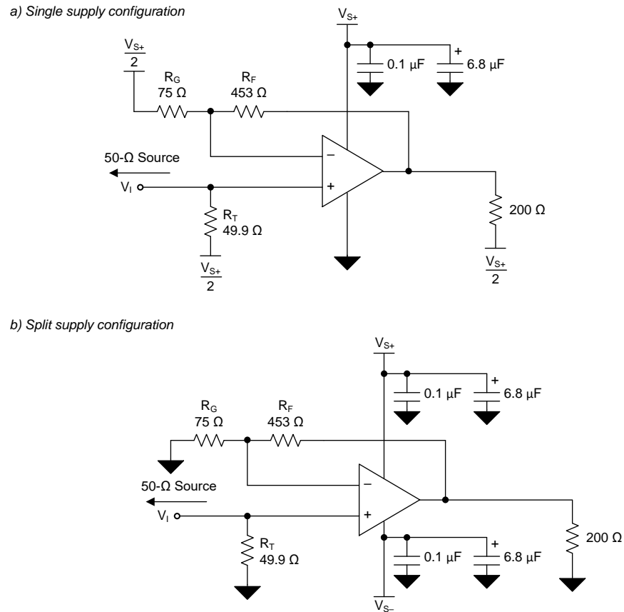
图 63. Split and Single Supply Circuit Configuration
