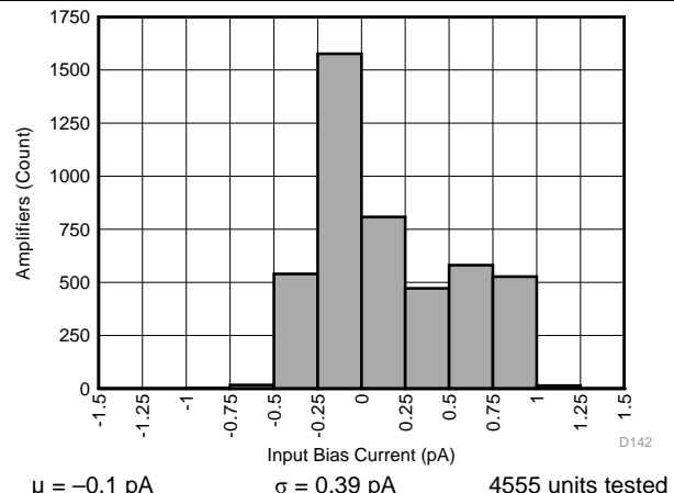
图 42. Input Bias Current Distribution
