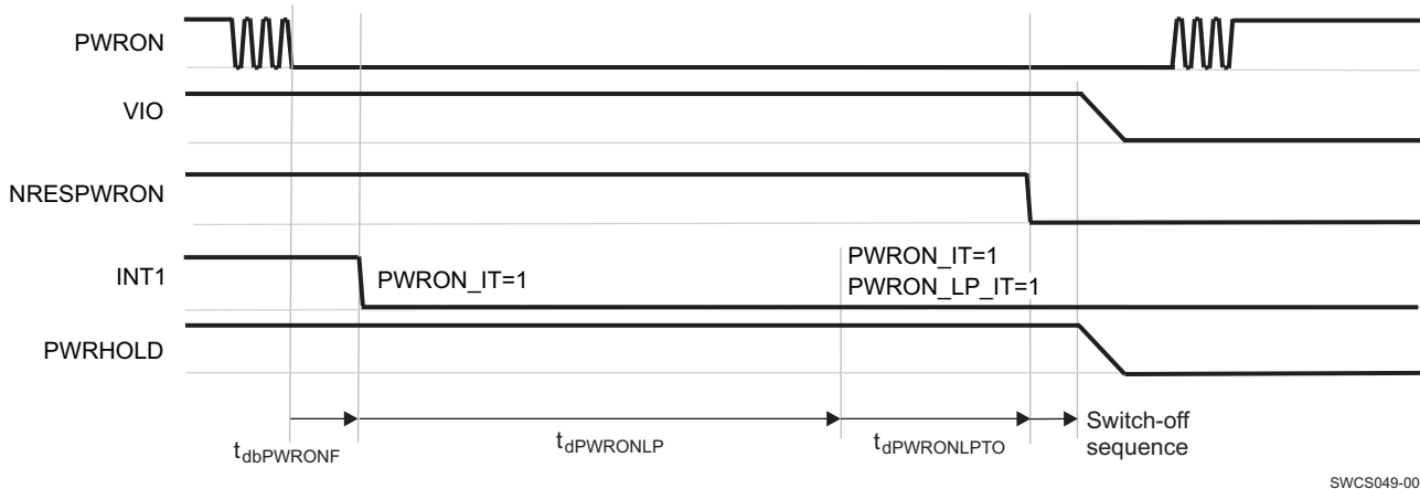
图 3. PWRON Long-Press Turn-Off
