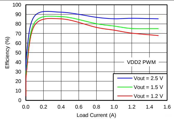
图 13. VDD2 Efficiency vs Load Current, 25°C, V_{IN} = 4 V, PWM
