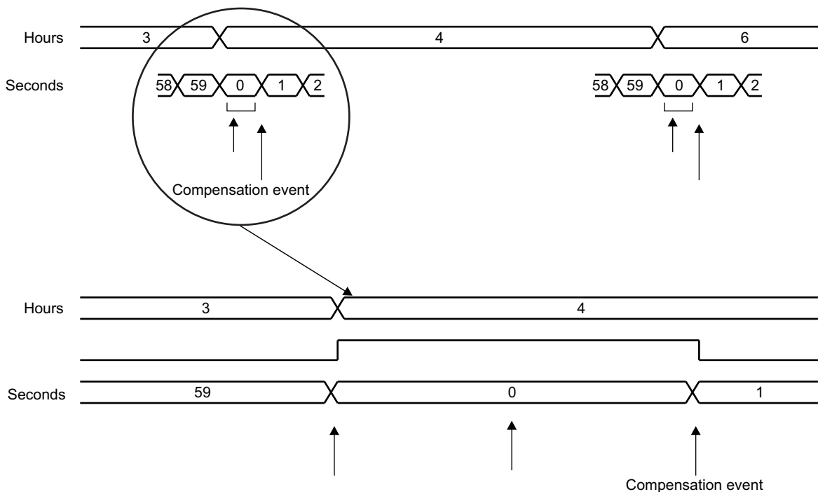
图 20. RTC Compensation Scheduling
