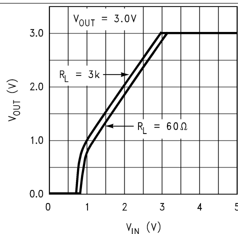
Figure 6. Dropout Characteristics
