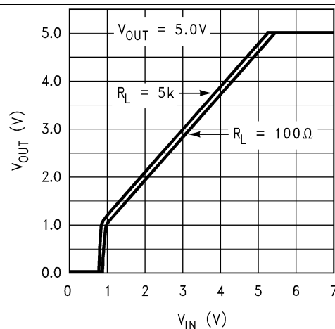
Figure 4. Dropout Characteristics
