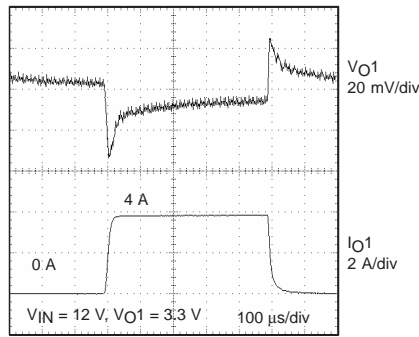
SBRC CH1 LOAD TRANSIENT RESPONSE
