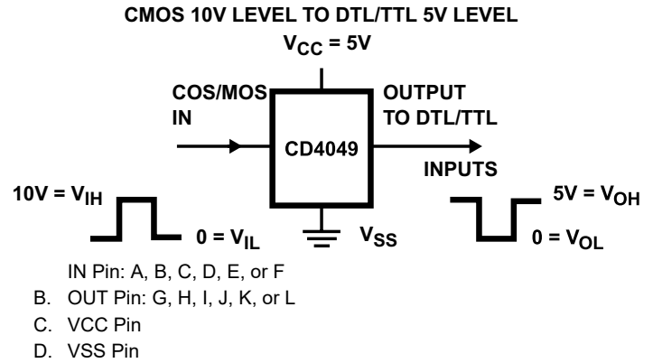
Figure 7-4. Logic Level Conversion Application
