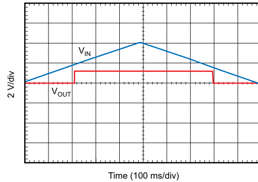
图 52. V_{IN} Ramp Up, Ramp Down Response
