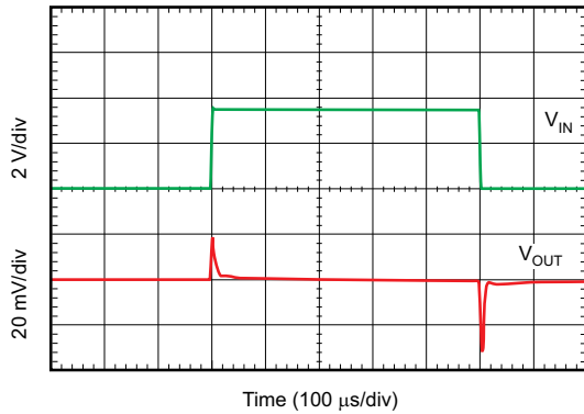
图 51. Line Transient Response
