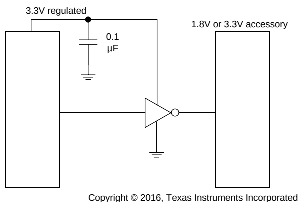
Figure 3. Typical Application Schematic
