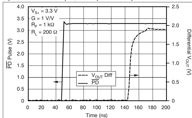
Figure 19. Turn-On Time
