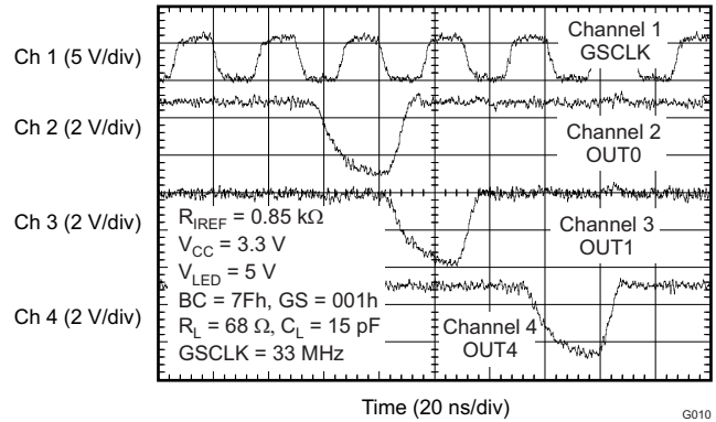
Figure 21. CONSTANT-CURRENT OUTPUT VOLTAGE WAVEFORM G010
