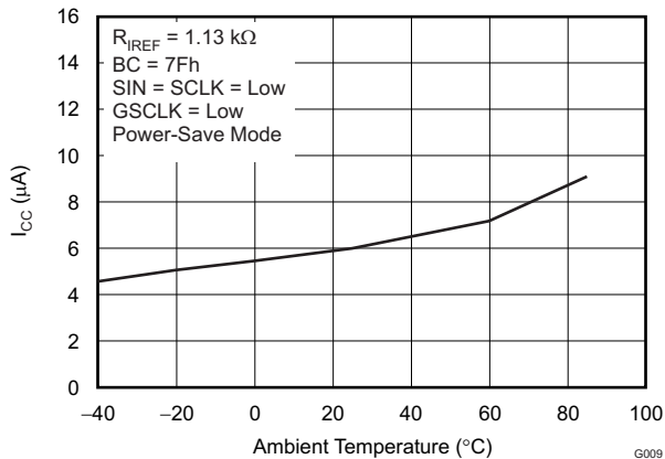
Figure 20. SUPPLY CURRENT IN POWER-SAVE MODE vs AMBIENT TEMPERATURE G009
