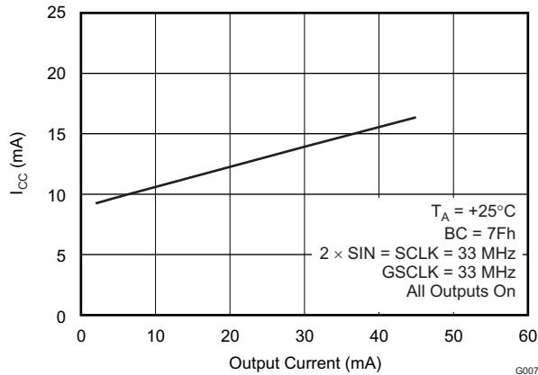
Figure 18. SUPPLY CURRENT vs OUTPUT CURRENT G007
