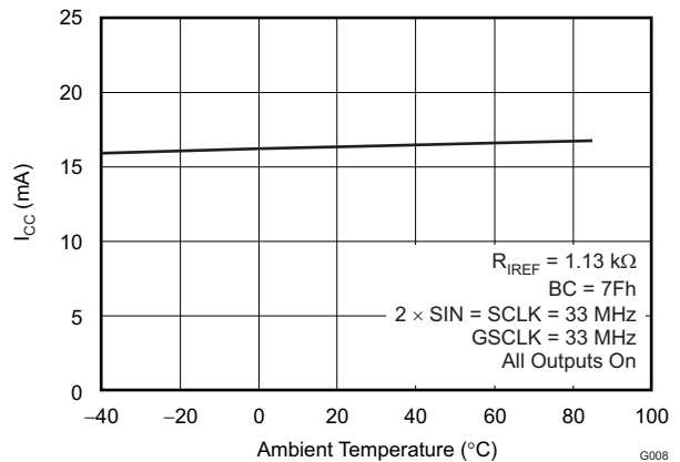
Figure 19. SUPPLY CURRENT vs AMBIENT TEMPERATURE G008
