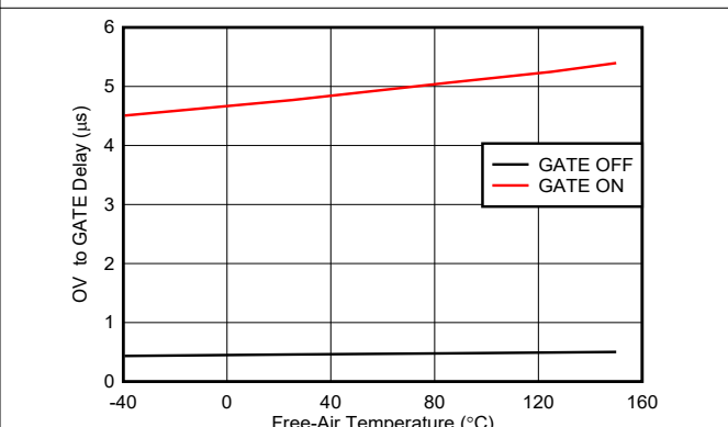
图 6-12. OV to GATE Delay vs Temperature (LM74502H)
