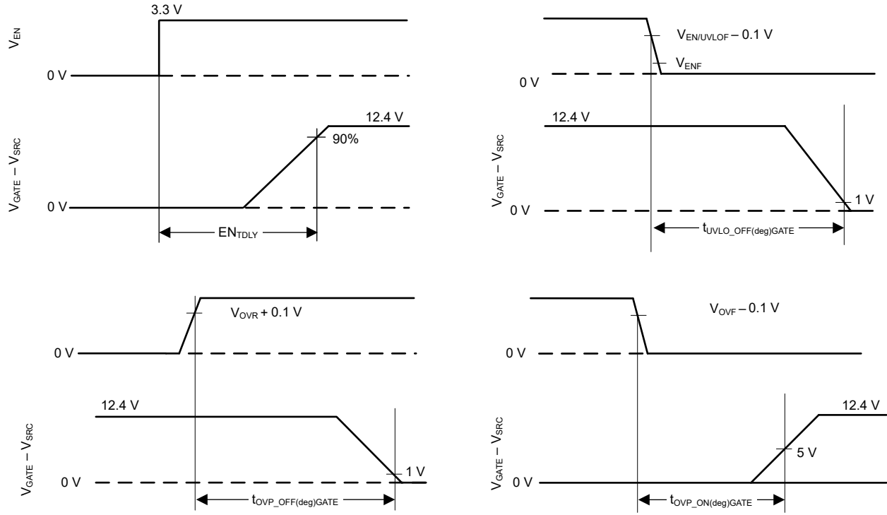
图 7-1. Timing Waveforms
