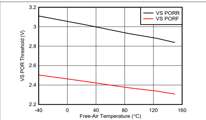
图 6-10. VS POR Threshold vs Temperature
