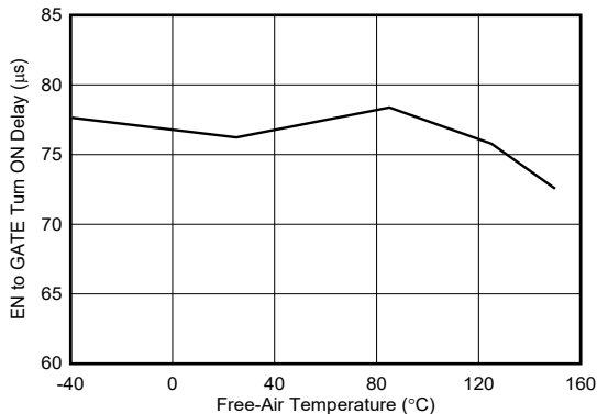
图 6-7. Enable to Gate Delay vs Temperature (LM74502H)
