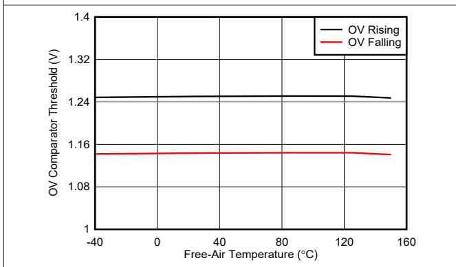
图 6-11. OV Comparator Threshold vs Temperature
