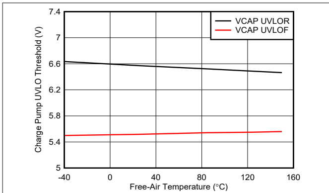
图 6-9. Charge Pump UVLO Threshold vs Temperature
