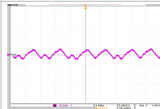
V_{OUT} = 3.3\text{ V} PFM T_A = 25^\circ\text{C} I_{OUT} = 0.5\text{ A} V_{IN} = 5.0\text{ V} BW = 20 MHz
