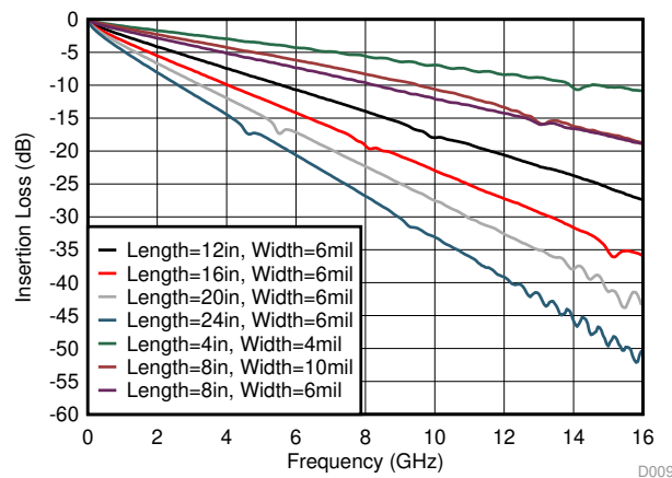
图 30. Insertion Loss of FR4 PCB Traces
