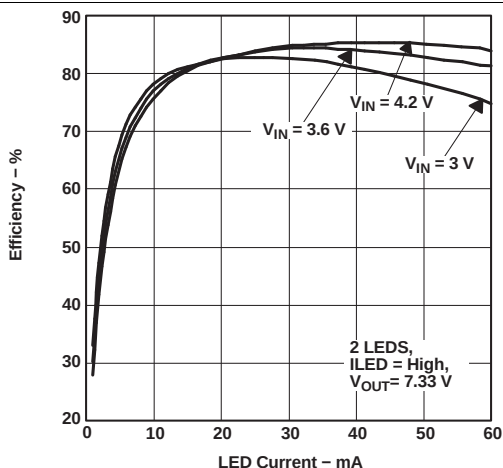
Figure 1. Efficiency vs LED Current
