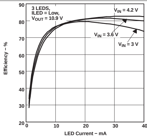
Figure 2. Efficiency vs LED Current
