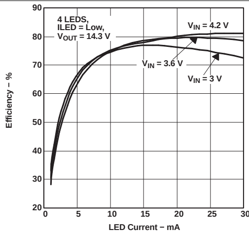
Figure 4. Efficiency vs LED Current
