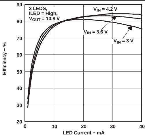
Figure 3. Efficiency vs LED Current
