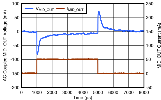
图 6-31. Load Transient (MID_OUT)
