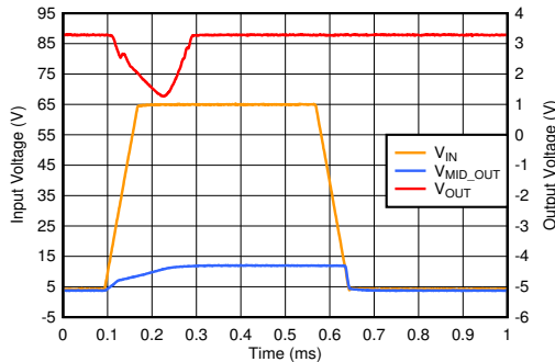
图 6-25. Line Transient ( V_{MID\_OUT} in Dropout)
