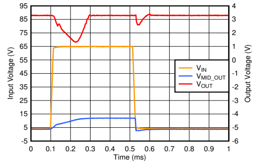
图 6-26. Line Transient ( V_{MID\_OUT} in Dropout)
