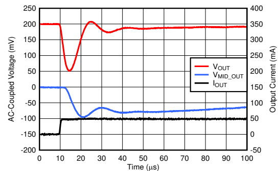
图 6-28. Load Transient (Rising Edge)
