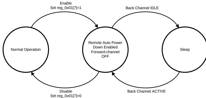
Figure 16. Remote Auto Power Down Sleep/Wake Cycle
