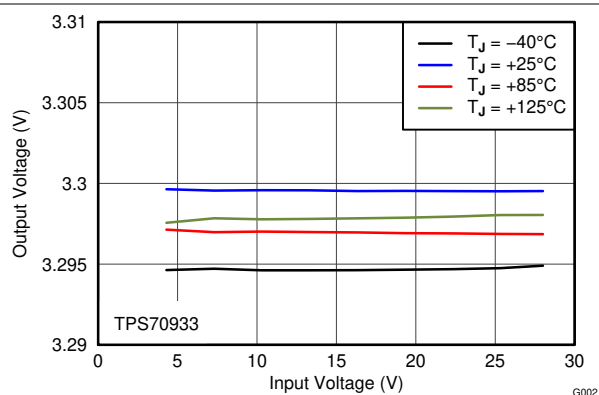
图 6-2. 3.3-V Line Regulation vs V_{\text{IN}} and Temperature
