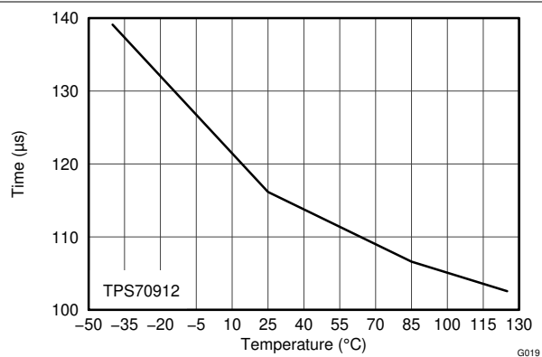
图 6-20. Start-Up Time vs Temperature
