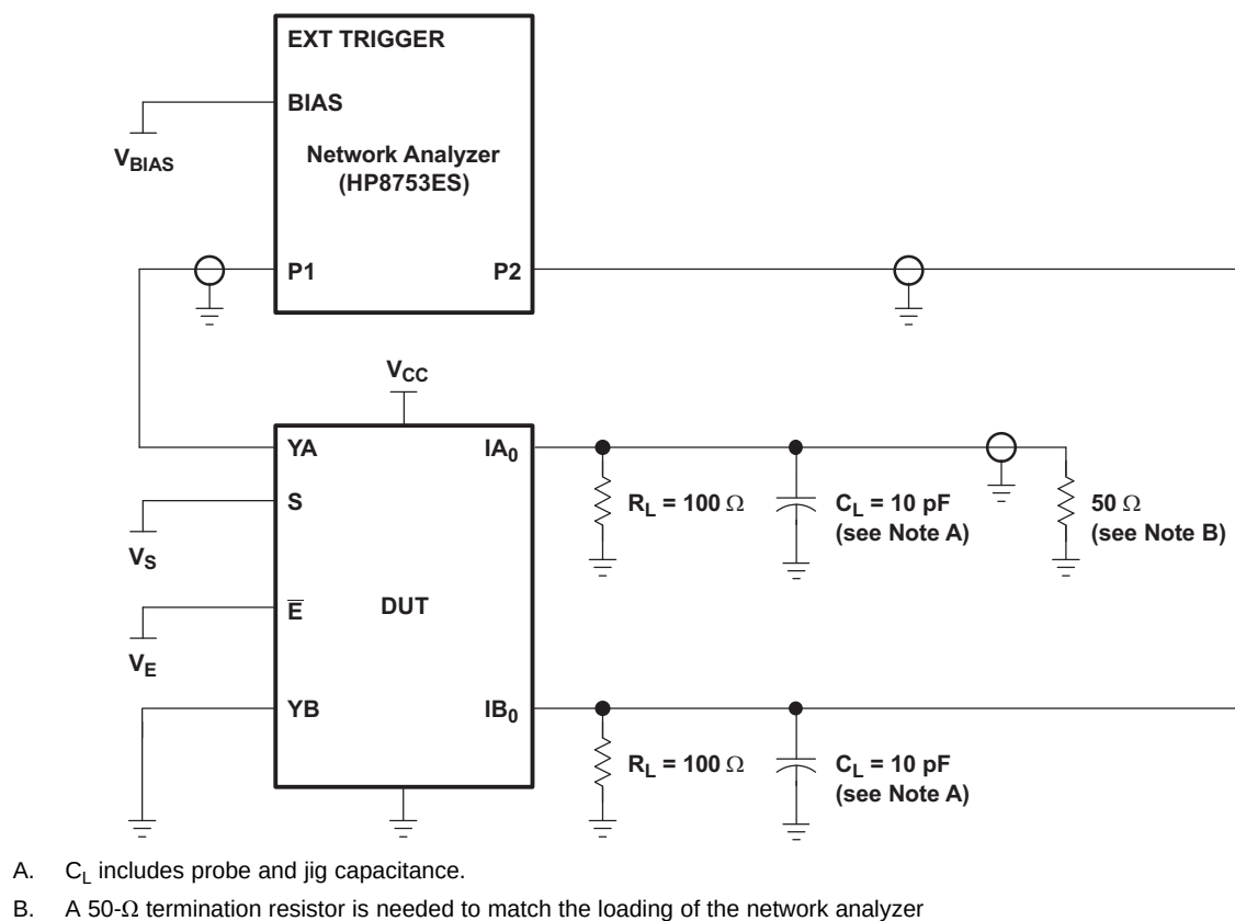
Figure 8. Test Circuit for Crosstalk ( X_{TALK} )
