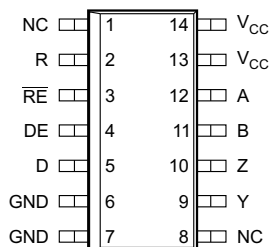
D Package 14-Pin SOIC SN65VD1791, 1792, 1793 Top View
