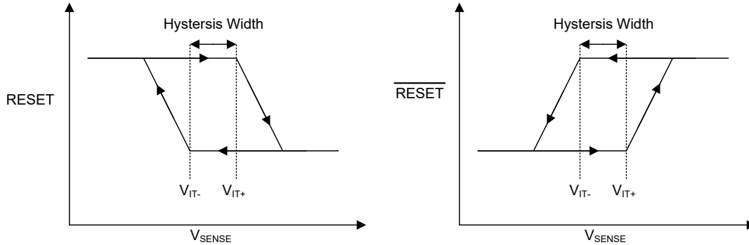
Figure 8-3. Hysteresis Diagram
