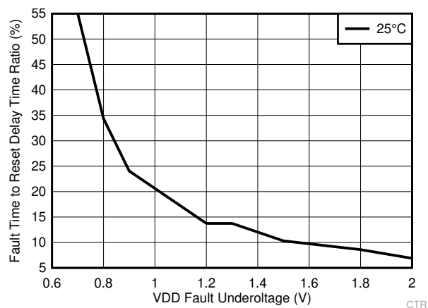
Figure 8-5. C_{CT\_EXT} Discharge Time During Fault Condition ( C_{CT\_EXT} = 1\ \mu\text{F} )
