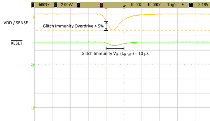
Figure 9-5. TLV841EVM SENSE Pin Glitch Immunity ( t_{GI\_VIT-} )
