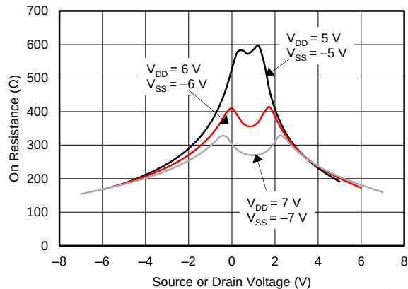
图 1. On-Resistance vs Source or Drain Voltage
