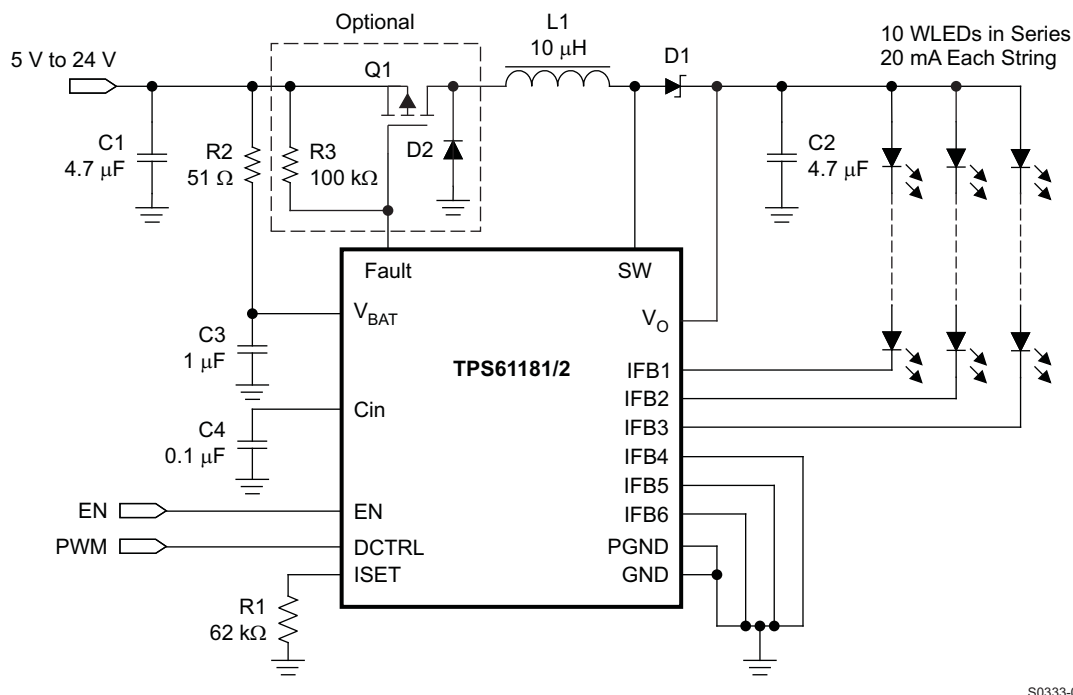
Figure 19. TSP61181/2 for Three Strings of LEDs
