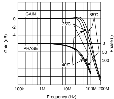
Closed Loop Frequency Response for Various Temperature
