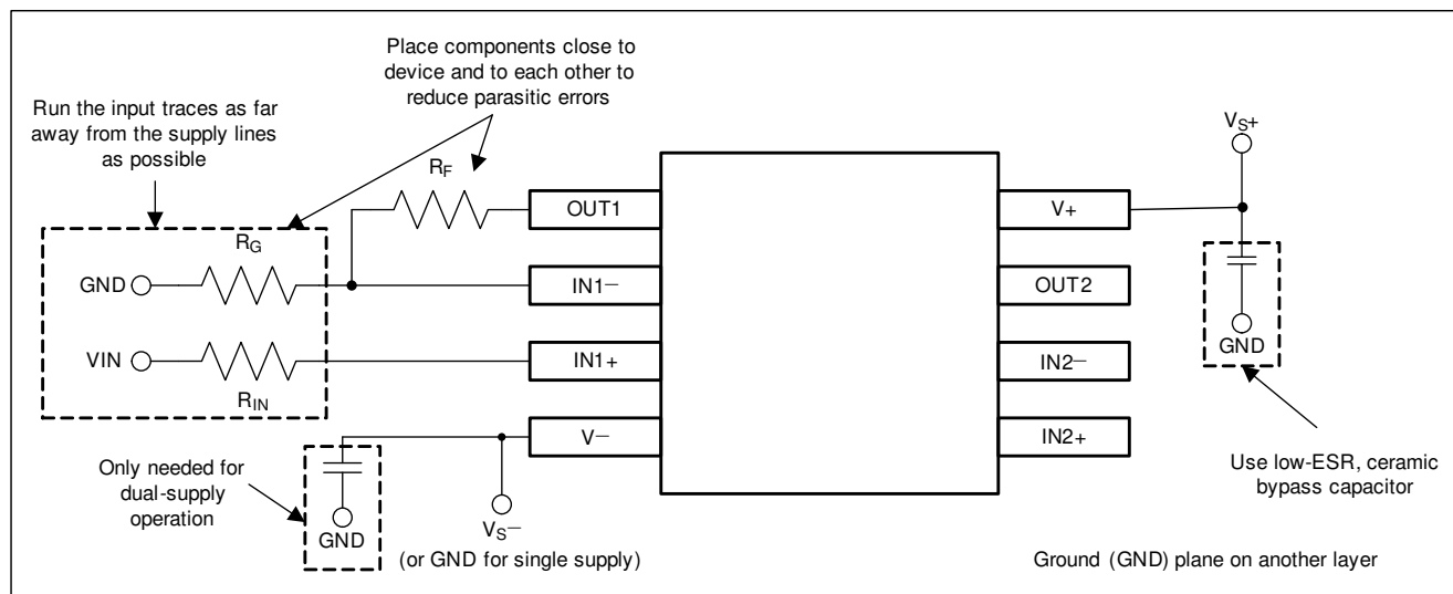
图 44. Operational Amplifier Board Layout for Noninverting Configuration
