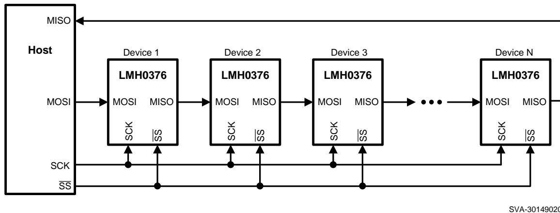
Figure 7. SPI Daisy Chain System Architecture
