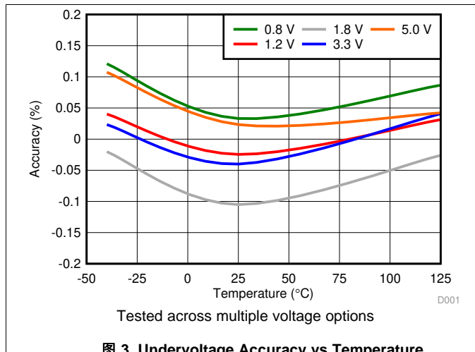
图 3. Undervoltage Accuracy vs Temperature
