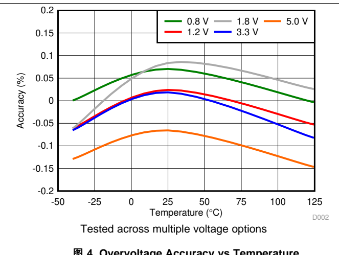
图 4. Overvoltage Accuracy vs Temperature
