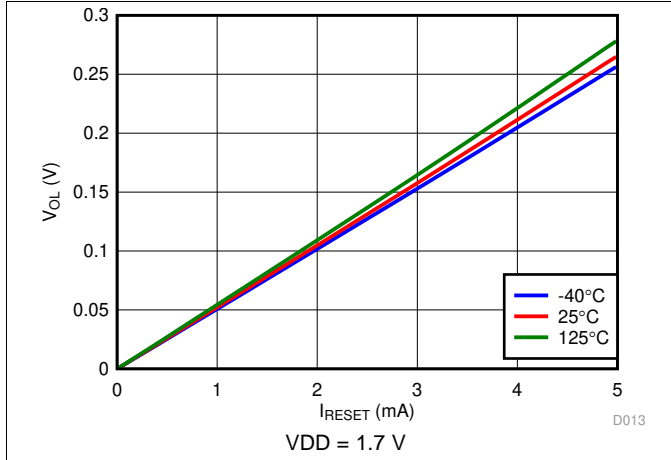
图 15. Low-Level Output Voltage vs RESET current
