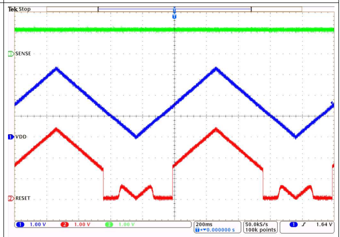
V_{DD} ramp from 0 V to 3.3 V, V_{SENSE} = 1.2 V, CT = OPEN V_{RESET} = V_{DD} = 3.3 V, TPS3703A4120
