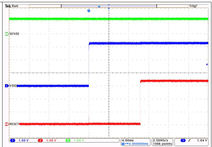
V_{DD} Start up from 0 V to 3.3 V, V_{SENSE} = 1.2 V, CT = OPEN V_{RESET} = V_{DD} = 3.3 V, TPS3703A4120
