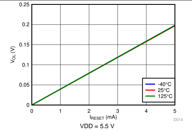
图 16. Low-Level Output Voltage vs RESET current
