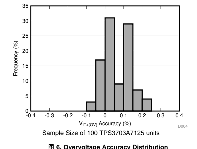
图 6. Overvoltage Accuracy Distribution
