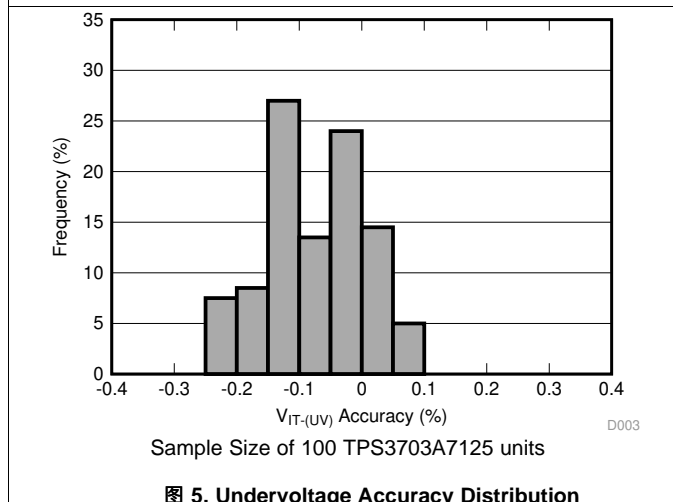
图 5. Undervoltage Accuracy Distribution
