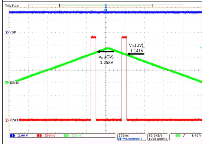
V_{SENSE} ramp from 0 V to 1.4 V, V_{DD} = 3.3 V, CT = OPEN V_{RESET} = V_{DD} = 3.3 V, TPS3703A4120
