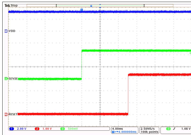
V_{SENSE} Start up from 0 V to 1.2 V, V_{DD} = 3.3 V, CT = OPEN V_{RESET} = V_{DD} = 3.3 V, TPS3703A4120
