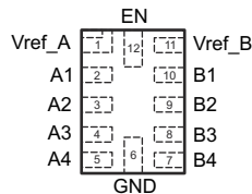
图 6-3. RUT Package 12-Pin UQFN Transparent Top View
