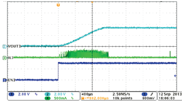
Figure 35. PSM Mode Buck3, Soft-Start With No Load
