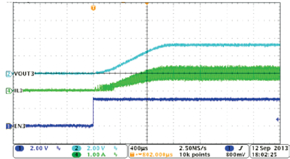
Figure 36. PSM Mode Buck3, Soft-Start With Full Load
