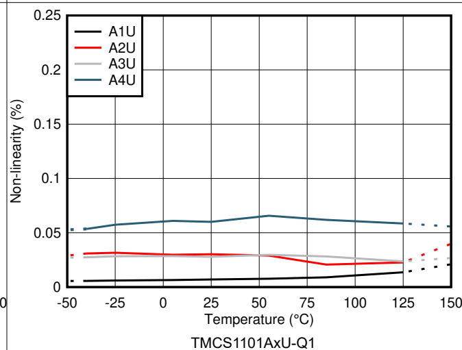
图 7-6. Non-Linearity vs. Temperature
