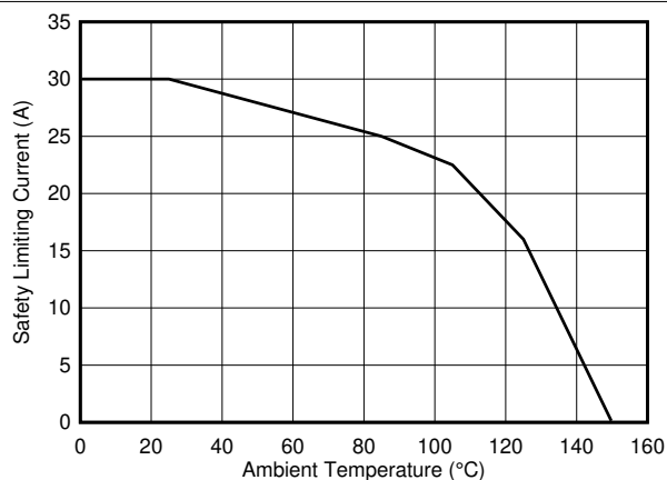
图 7-28. Thermal Derating Curve for Safety-Limiting Current, Side 1
