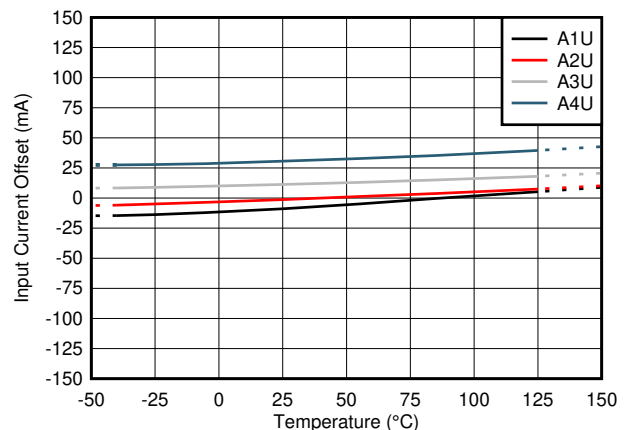
图 9-3. Offset Error Drift Across Temperature (U Variants)
