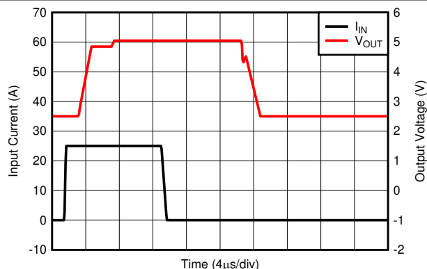
图 7-25. Current Overload Response
