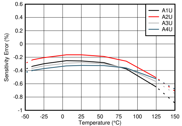
图 9-5. Sensitivity Drift Across Temperature (U Variants)
