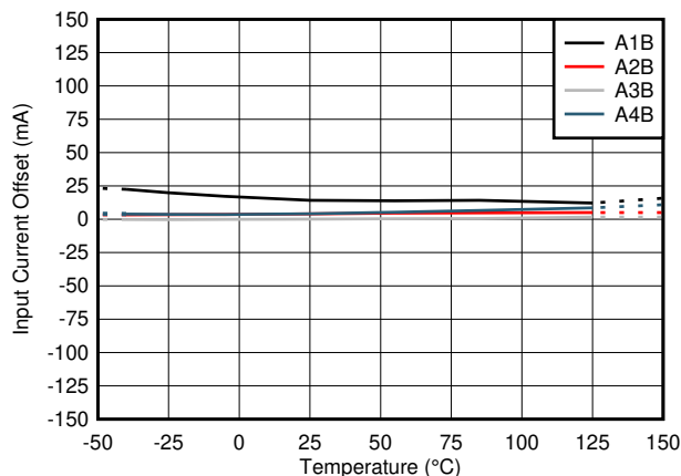
图 9-2. Offset Error Drift Across Temperature (B Variants)
