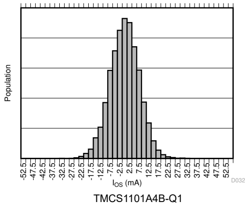
图 7-15. Input Offset Current Production Distribution
