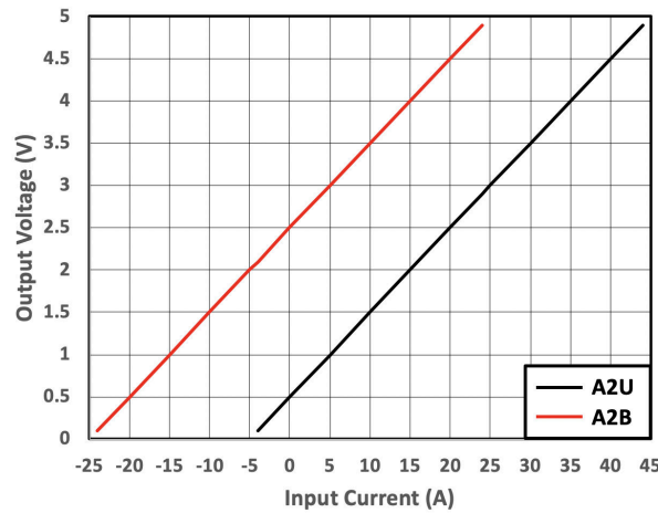
图 9-14. Output Voltage Relationship to Input Current for TMCS1101A2B-Q1 and TMCS1101A2U-Q1
