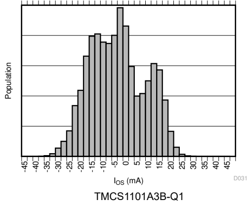
图 7-13. Input Offset Current Production Distribution
