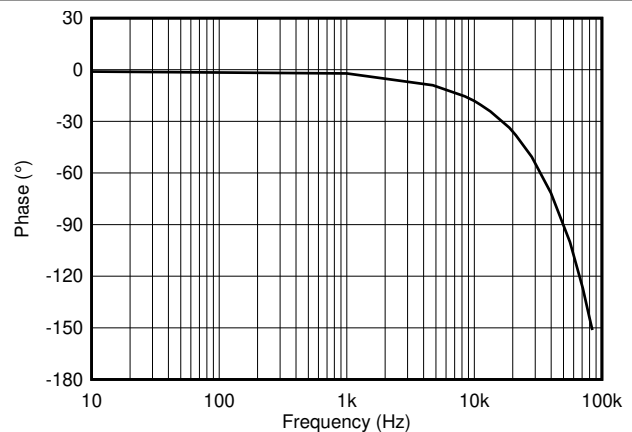
图 7-18. Phase vs. Frequency, All Gains
