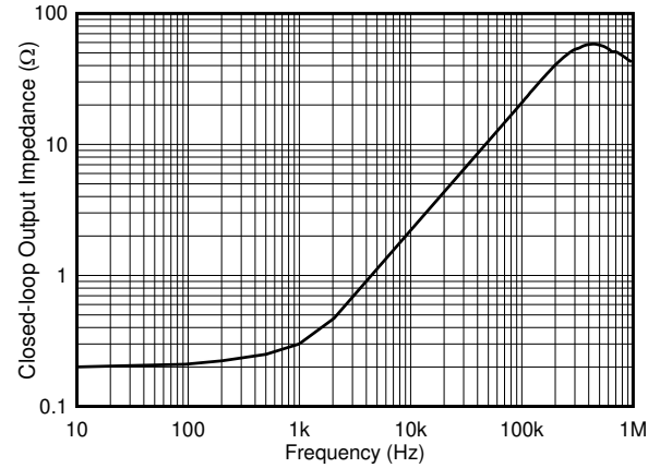
图 7-20. Output Impedance vs. Frequency
