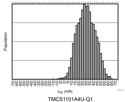
图 7-16. Input Offset Current Production Distribution
