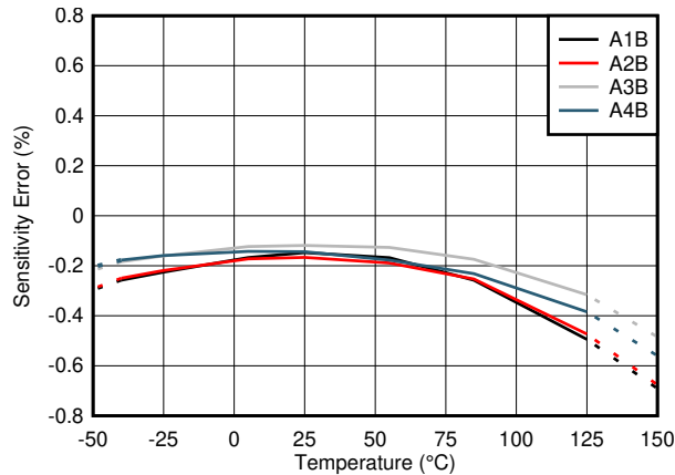
图 9-4. Sensitivity Drift Across Temperature (B Variants)
