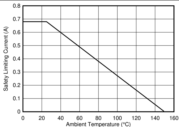
图 7-29. Thermal Derating Curve for Safety-Limiting Current, Side 2
