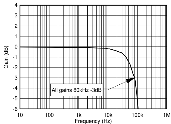
图 7-17. Sensitivity vs. Frequency, All Gains Normalized to 1 Hz
