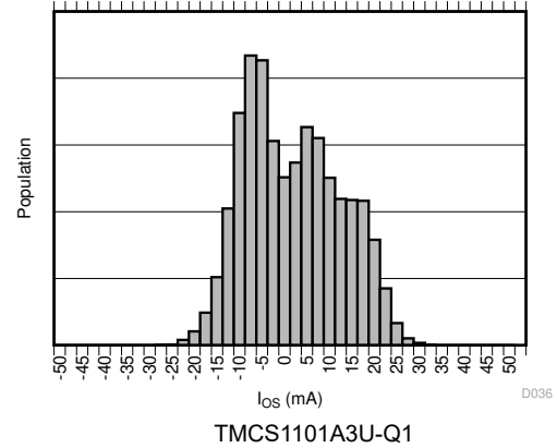
图 7-14. Input Offset Current Production Distribution
