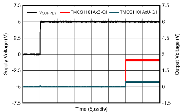
图 7-26. Startup Transient Response
