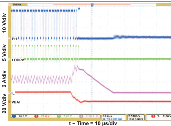
Figure 9. Battery Insertion
