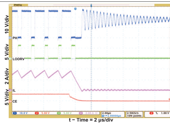
Figure 2. Charge Enable
