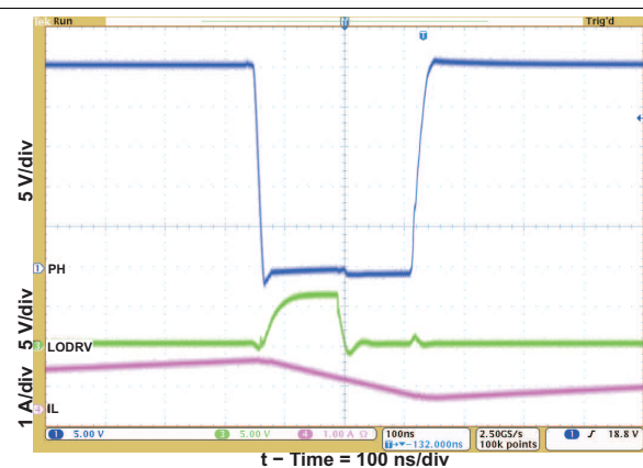
Figure 4. Charge Disable
