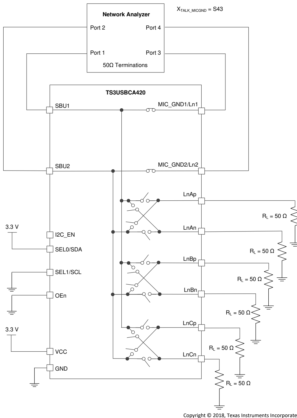
图 12. Crosstalk Between MIC and AGND (XTALK MICGND )
