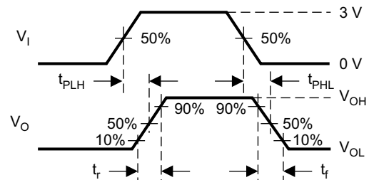
图 20. Measurement of Receiver Output Rise and Fall Times and Propagation Delays
