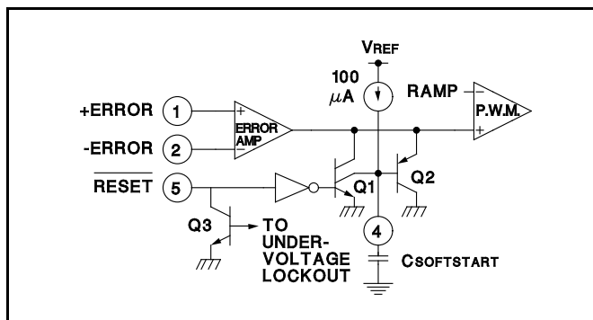
Figure 3. Soft-Start Circuit Schematic
