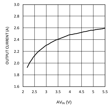
Figure 10. Maximum Sourcing Current vs AV_{IN} ( V_{DDQ} = 2.5 V, PV_{IN} = 2.5 V)
